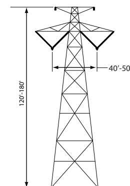
Self-Supporting V-String Structure
