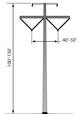
Tubular Pole V-String Structure
